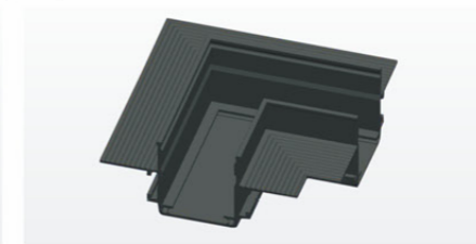
名称/Name: L形预埋磁吸导轨接头 L-shaped embedded magnetic guide rail joint 材质/Material: 铝材/Aluminum 颜色/Colour: 砂白、砂黑/White、Black 尺寸/Size: 100x100x68mm
