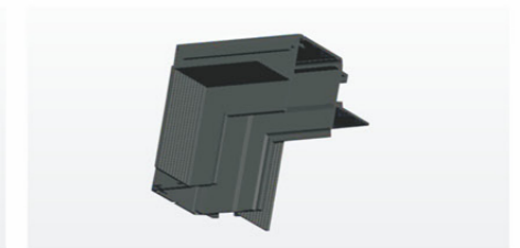
名称/Name: 7形预埋磁吸导轨接头 7-shaped embedded magnetic guide rail joint 材质/Material: 铝材/Aluminum 颜色/Colour: 砂白、砂黑/White、Black 尺寸/Size: 100x100x68mm
