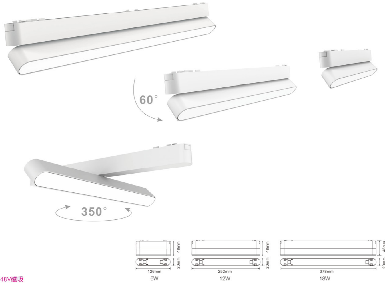
48V磁吸 48V Magnetic suction
